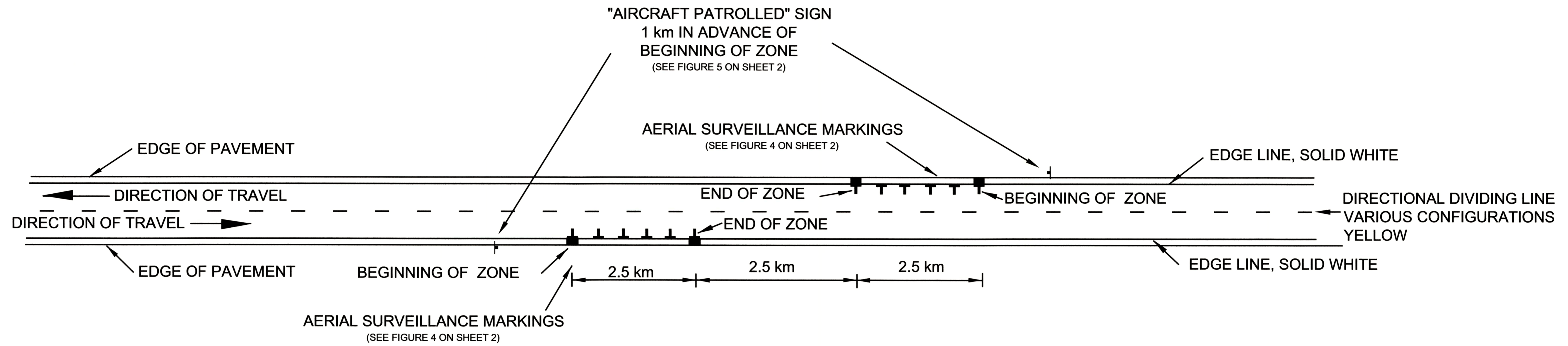
FIGURE 1 - TWO LANE TWO WAY HIGHWAY MARKED IN EACH DIRECTION
