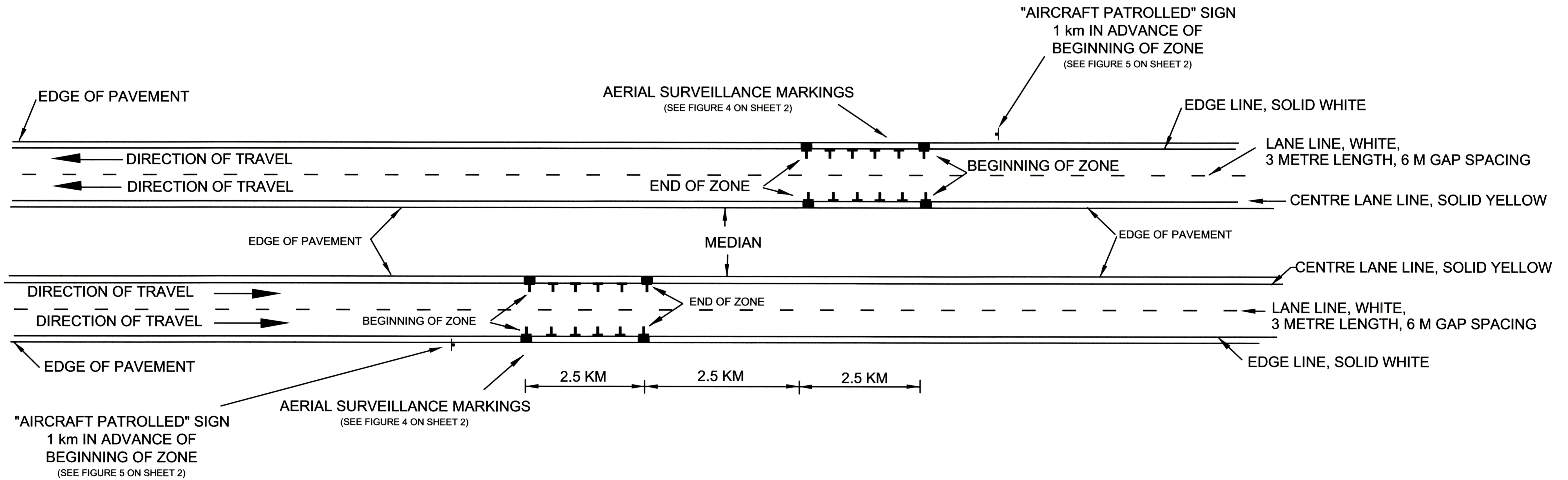
FIGURE 2 - MULTILANE HIGHWAY SEPARATED BY MEDIAN MARKED IN EACH DIRECTION
